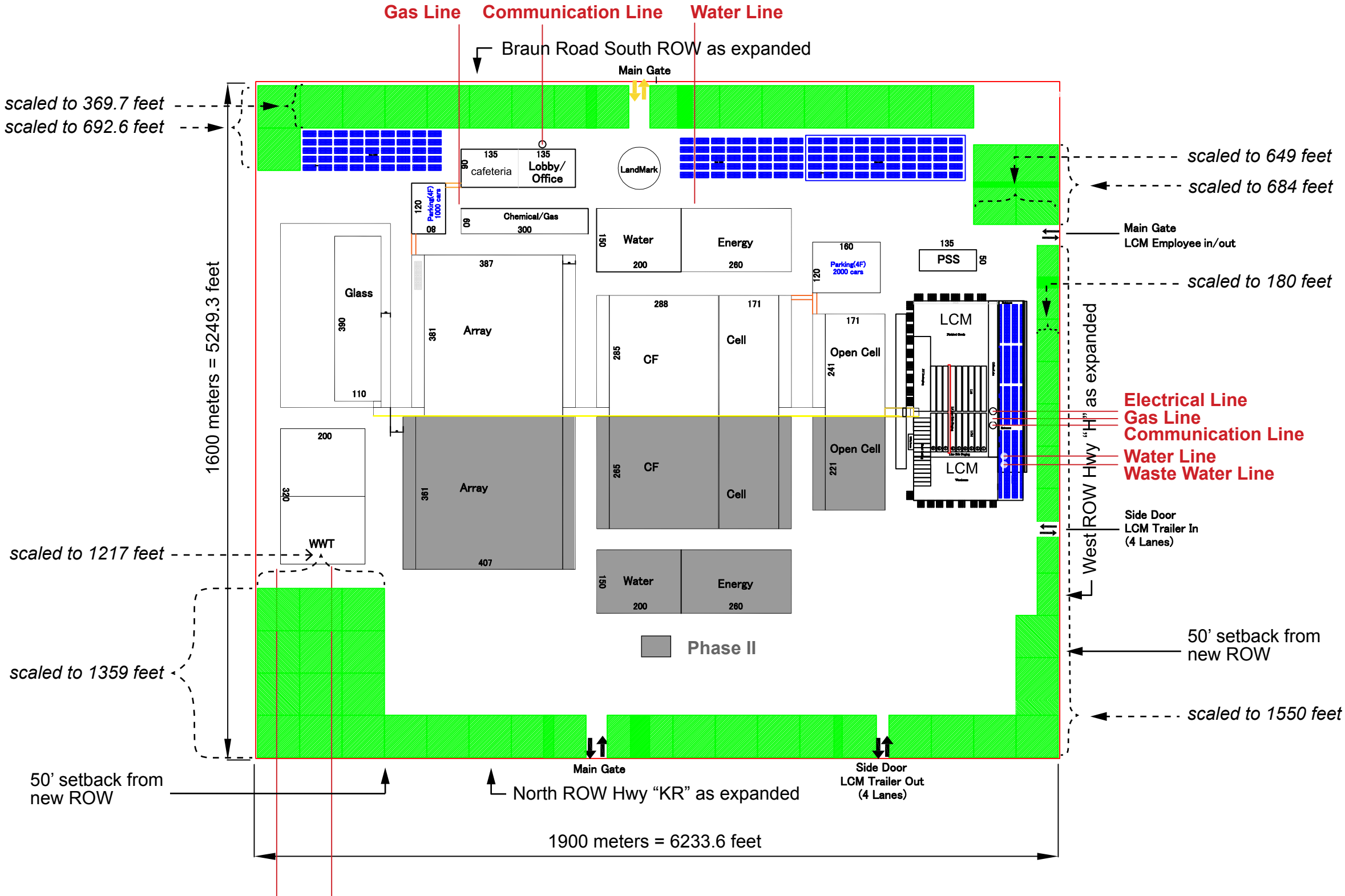
Phase I Site Plan for Facility draft dated 11-30-2017
